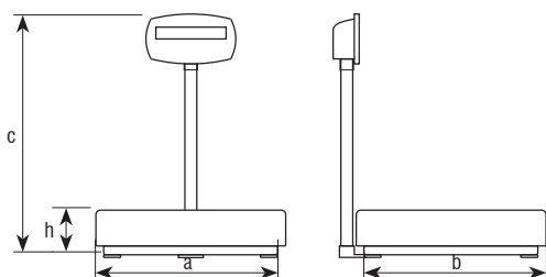
Dimensions (mm)
